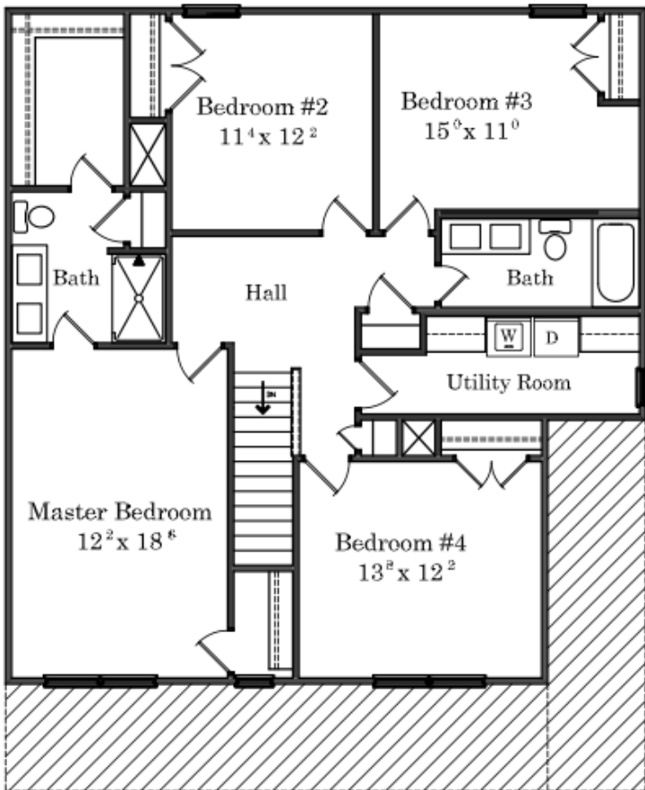
SECOND FLOOR
