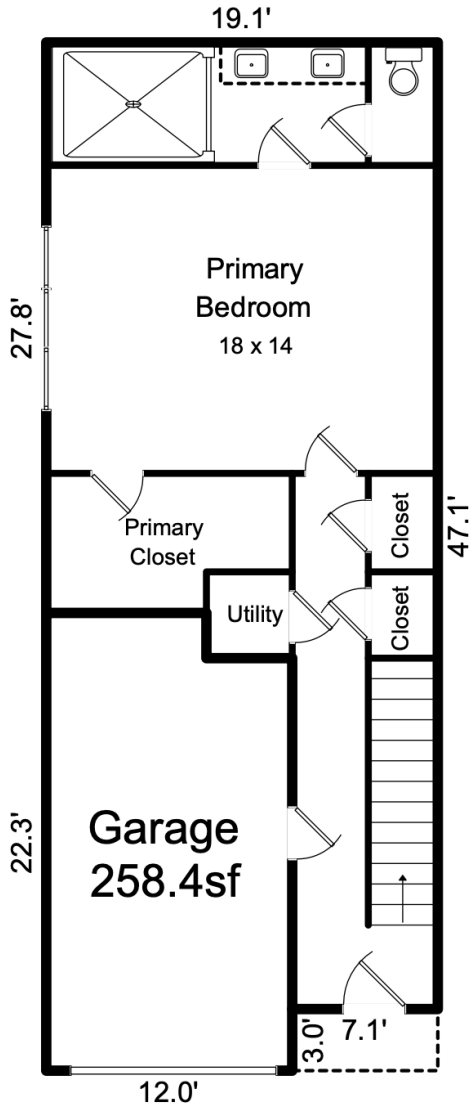
First Floor 677.3sf
