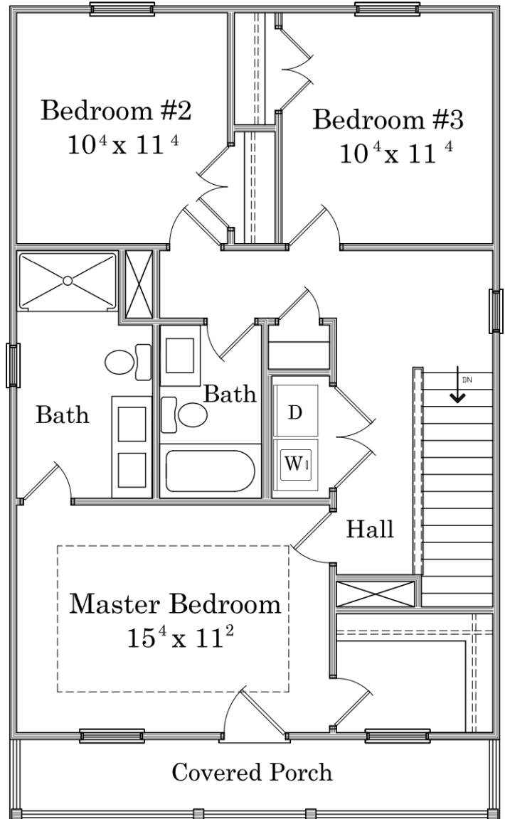
SECOND FLOOR
